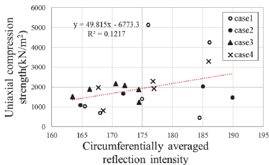
Fig.6 Relationship between circumferentially averaged reflection intensity and uniaxial compression strength
